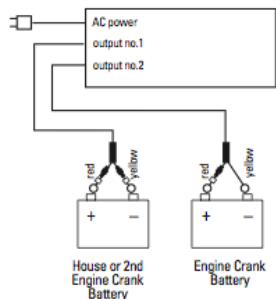
Fig. 7 ProSport 8, 12, & 20 Dual Output Charger for 2 Batteries Typical
