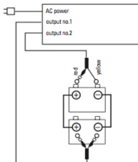
Fig. 6 ProSport 8, 12, & 20 Dual Output Charger for 2 Batteries Typical
