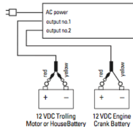
Fig. 1 ProSport 6, 12, & 20 Dual Output Charger for 2 Batteries Maximum Typical
