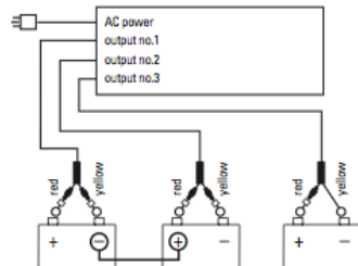
Fig. 2 ProSport 20 Plus Triple Output Charger for 3 Batteries Maximum Typical
