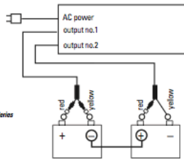
Fig. 4 ProSport 8, 12, & 20 Dual Output Charger for 2 Batteries Maximum Typical
