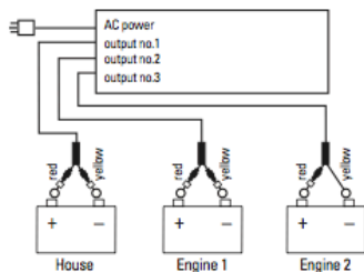
Fig. 8 ProSport20 Plus Triple Output Charger for 3 Batteries
