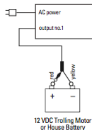
Fig. 3 ProSport 6 Single Output Charger for 1 Battery Maximum Typical
