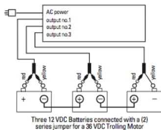
Fig. 5 ProSport20 Plus Triple Output Charger for 3 Batteries Maximum Typical
